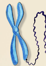
Chromosome
