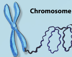
Chromosome
